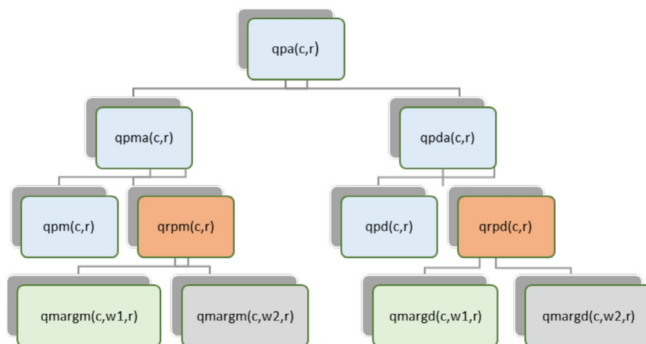
FIGURE 2 | Nesting structure for private household waste demands in MAGNET. Source: Bartelings and Philippidis (2024).
