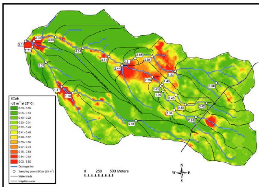
Figure 1 Raster map of apparent soil electrical conductivity (ECah) in the Barranco de Lerma study area. The delineation of the 25 watersheds within this area and the EC of the drainage waters (ECdw) at the exit of each watershed are also shown.
