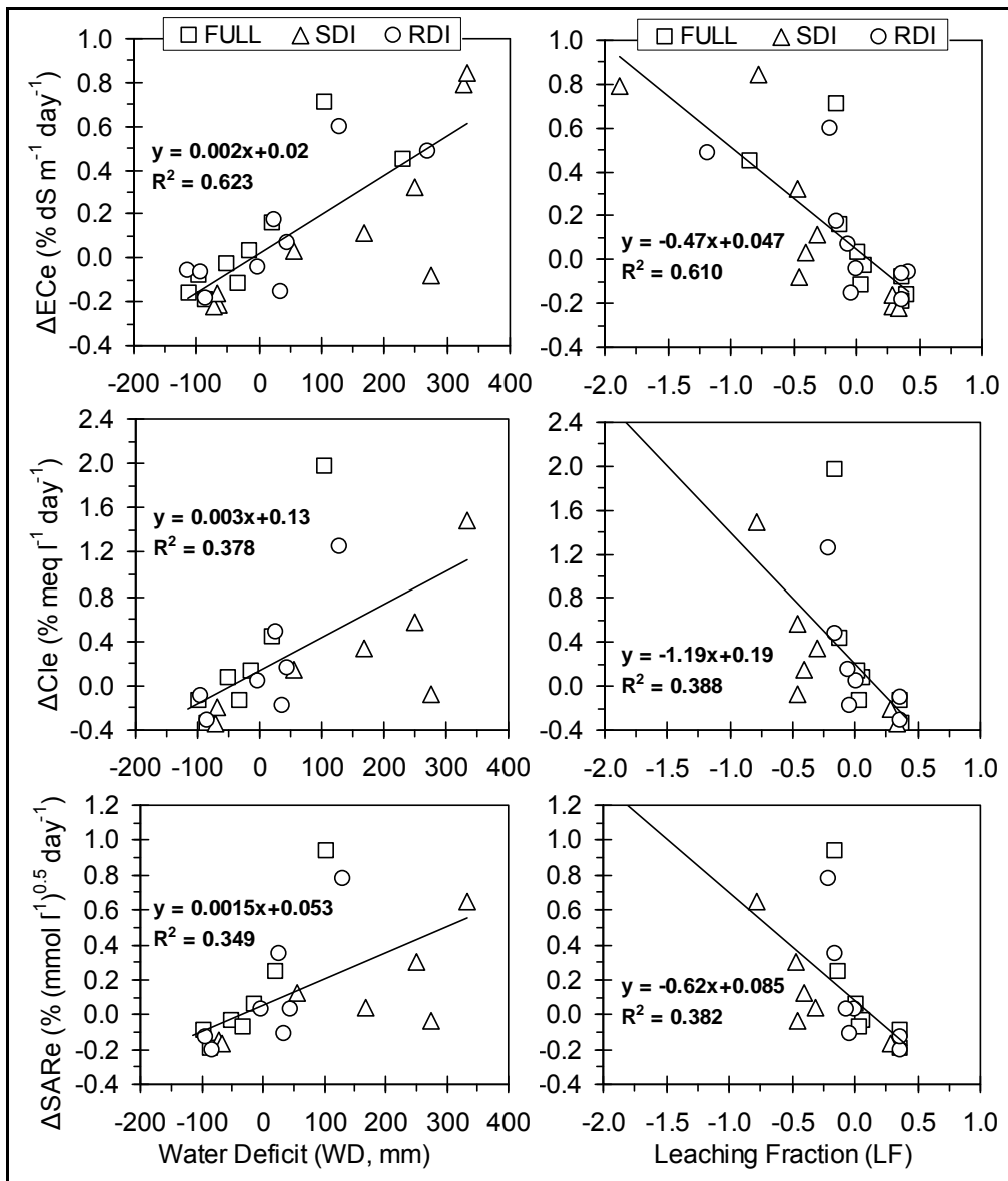
Fig. 4. Relationships and linear regression equations between changes in soil salinity ( \Delta E_{Ce} ), chloride concentration ( \Delta Cl_e ) and sodicity ( \Delta SAR_e ) measured between sampling dates, and field-wide Water Deficits (WD) and leaching fractions (LF) calculated for the periods between sampling dates. \Delta is given in terms of percent change per day at the end of each period between sampling dates relative to the values at the beginning.
