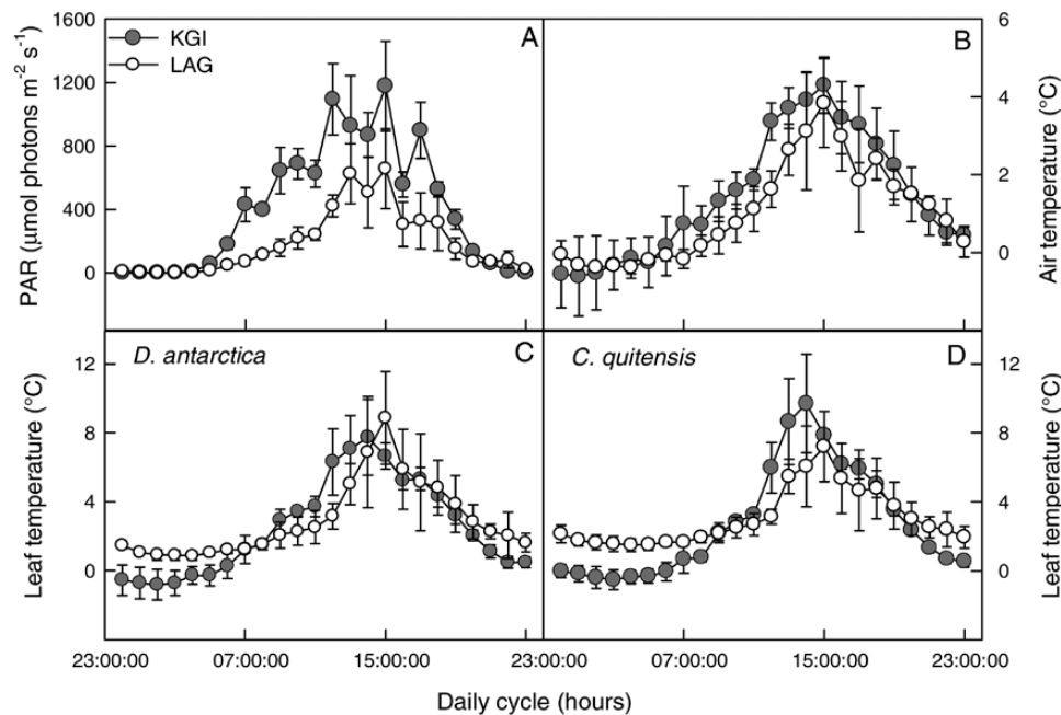
Fig. 2. Diurnal course of photosynthetically active radiation (A), air temperature (B), and leaf temperature in D. antarctica (C) and C. quitensis (D) in King George (KGI) and Lagotellerie Island (LAG) between 17 and 22 January 2015. Values are means ± SE
