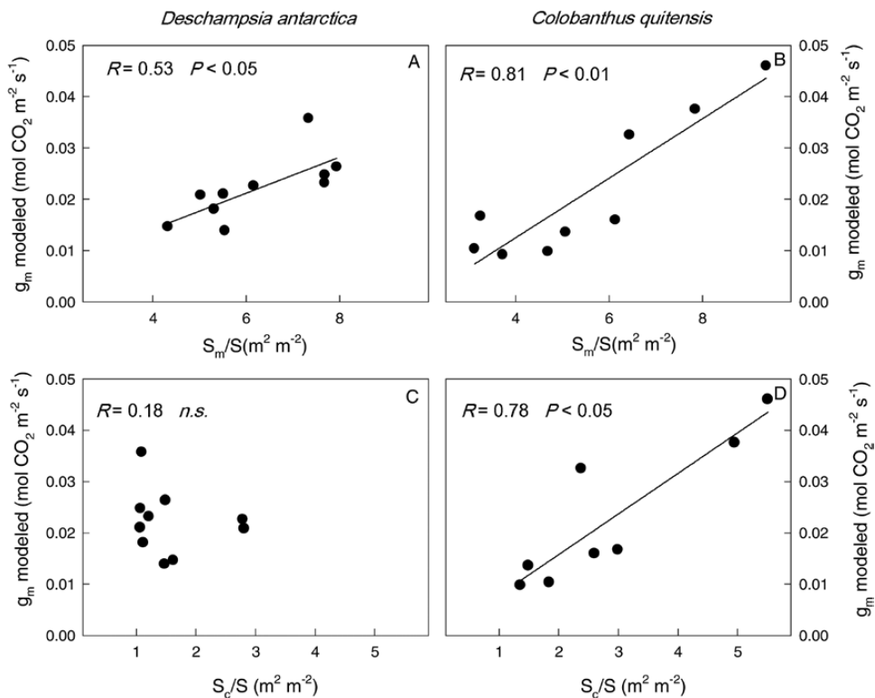
Fig. 6. Correlations of the leaf mesophyll conductance modeled with anatomical parameters ( g_m modeled) with the mesophyll ( S_m/S ) and chloroplast ( S_c/S ) surface area facing intercellular air spaces per leaf area in D. antarctica (left) and C. quitensis (right). The Pearson correlation coefficient and the significance of the relationship are shown for each species considering both populations together. Values are means \pm SE ( n=3-5 ).
