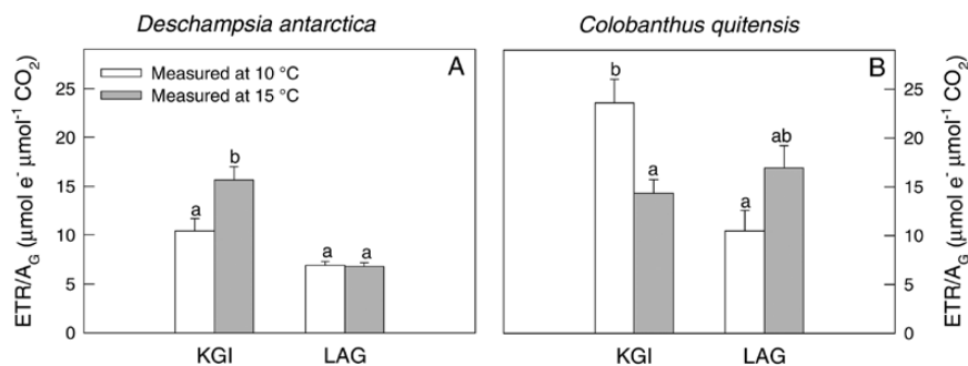
Fig. 7. The ratio of the electron transport rate and gross photosynthesis (ETR/A G ) for D. antarctica (A) and C. quitensis (B) in King George (KGI) and Lagotellerie Island (LAG), measured at 10 °C (white bars) or 15 °C (gray bars). Values are means ± SE ( n=5-7 ). Different letters indicate statistically significant differences for each species between populations and measurement temperatures according to Tukey ( P<0.05 ).
