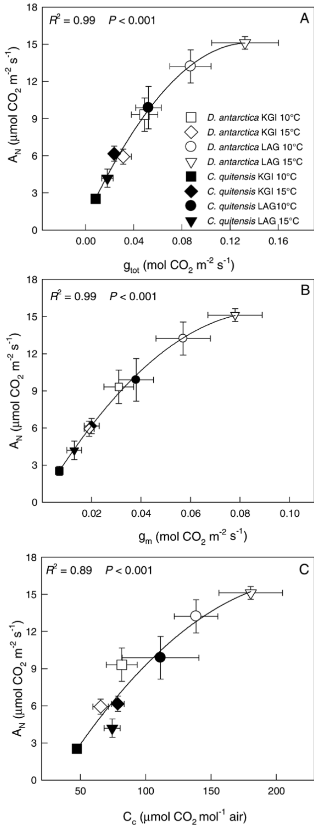
Fig. 5. The relationship of (A) the total leaf conductance ( g_{\text{tot}} ), (B) the leaf mesophyll conductance ( g_m ), and (C) the chloroplast CO 2 concentration ( C_c ) to the net photosynthetic CO 2 assimilation rate ( A_N ) of D. antarctica (open circles) and C. quitensis (filled circles) in King George (KGI) and Lagotellerie Island (LAG). Goodness of fit with a saturation model is shown for both species and considering all populations and measurement temperatures together. Values are means \pm SE ( n=5-7 ).
