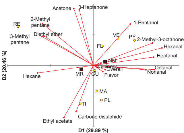
Figure 2. Biplot of the Principal Component Analysis of the volatile compounds of cooked meat of 8 breeds of kids fed natural milk (NM) or milk replacers (MR). FL: Florida; GU: del Guadarrama; MA: Majorera; PL: Palmera; PY: Payoya; RE: Retinta; TI: Tinerfeña; VE: Verata. The volatile compounds are expressed as percentage of total detected volatile compounds.
