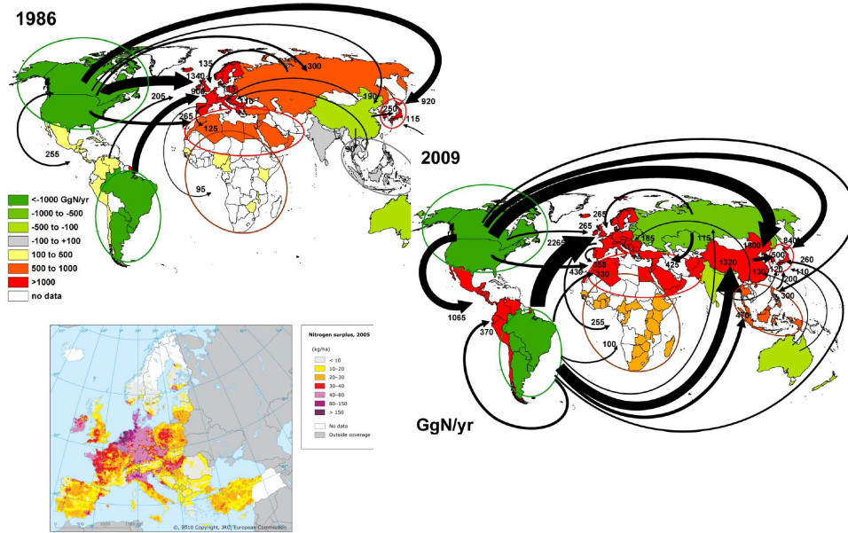
Fig. 3 N fluxes from each region to the others for the years 1986 and 2009. Arrows show the fluxes between the regions (only fluxes higher than 90 GgN are represented)
