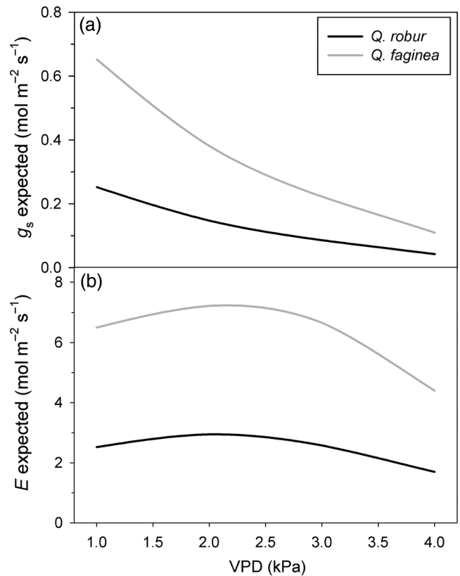
Figure 4. (a) Relationship between VPD and the expected stomatal conductance ( g_s ) and (b) relationship between VPD and the expected transpiration ( E ) for Q. robur and Q. faginea according to the empirical model given by Oren et al. (1999).
